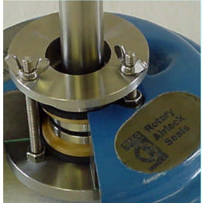
MECO-PAC in cutaway stuffing box
